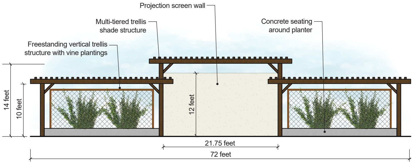
Trellis shade structure elevation.
